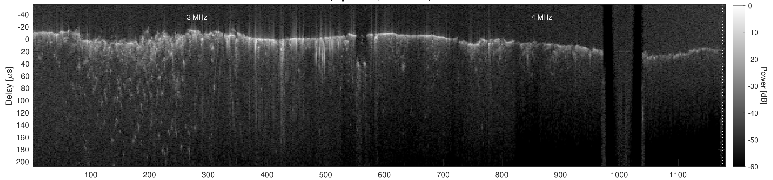
Orbit 10384, Cluttergram
