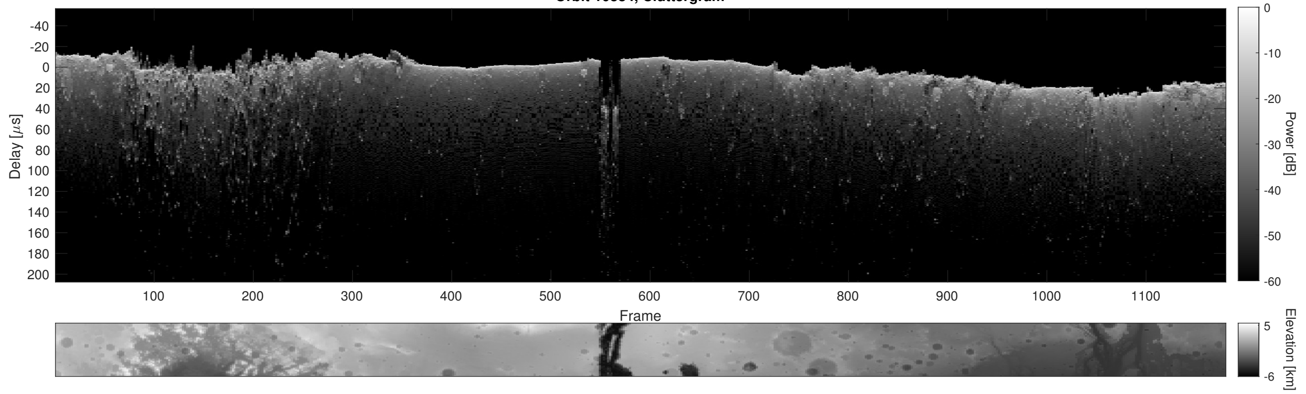
Orbit 10384, Cluttergram
