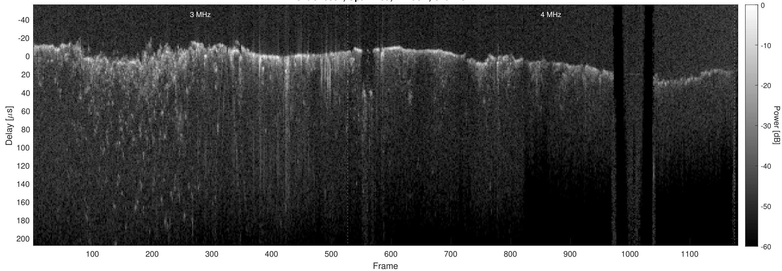
Orbit 10384, Optimized, Window, Channel 2
