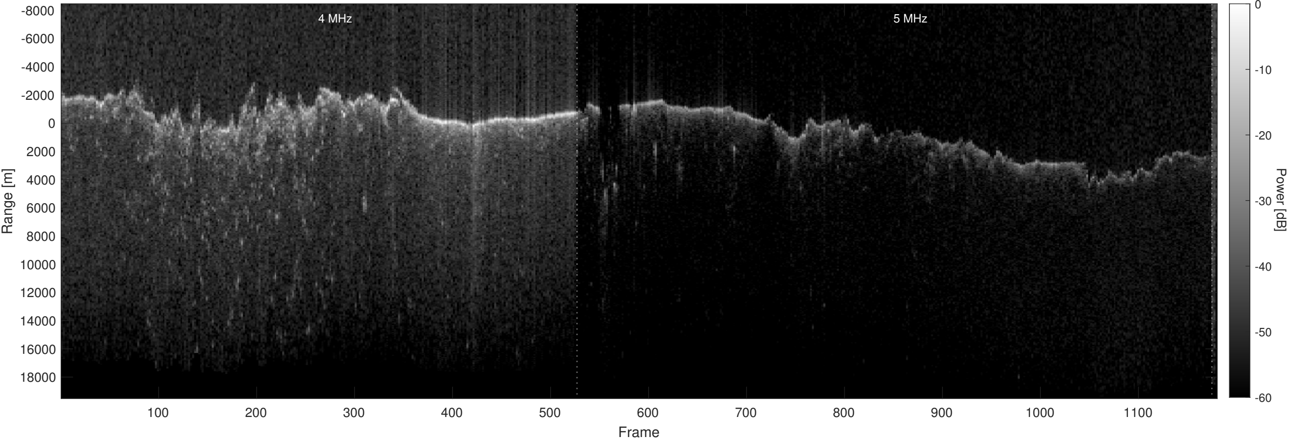
Orbit 10384, Optimized, Window, Depth-Corrected, Channel 2
