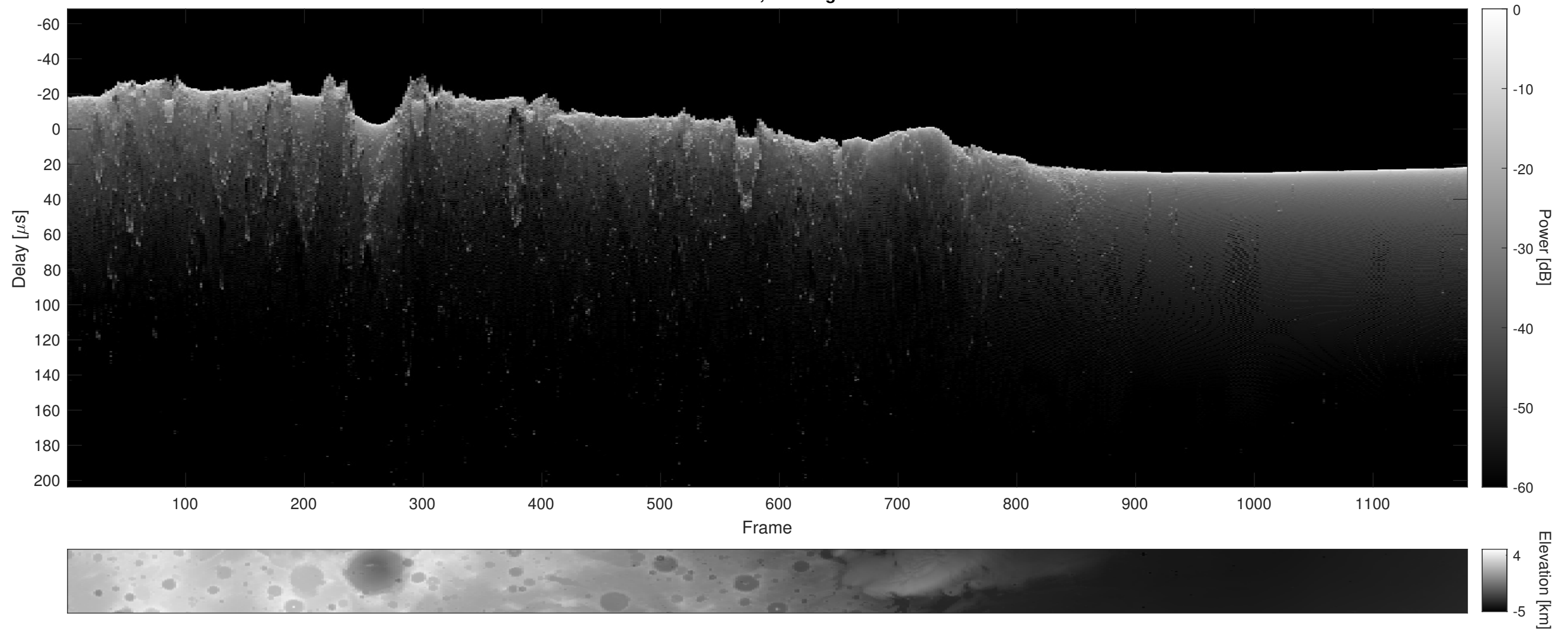
Orbit 10385, Cluttergram
