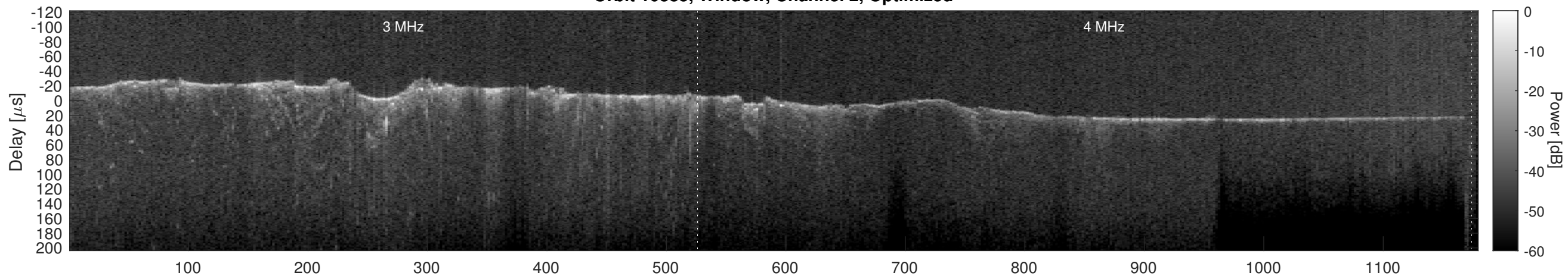
Orbit 10385, Cluttergram
