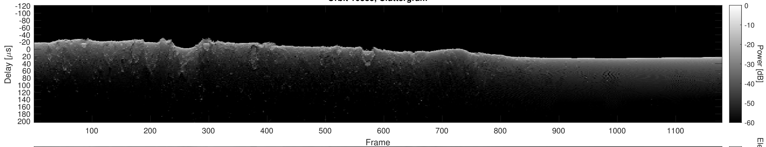
Orbit 10385, Cluttergram
