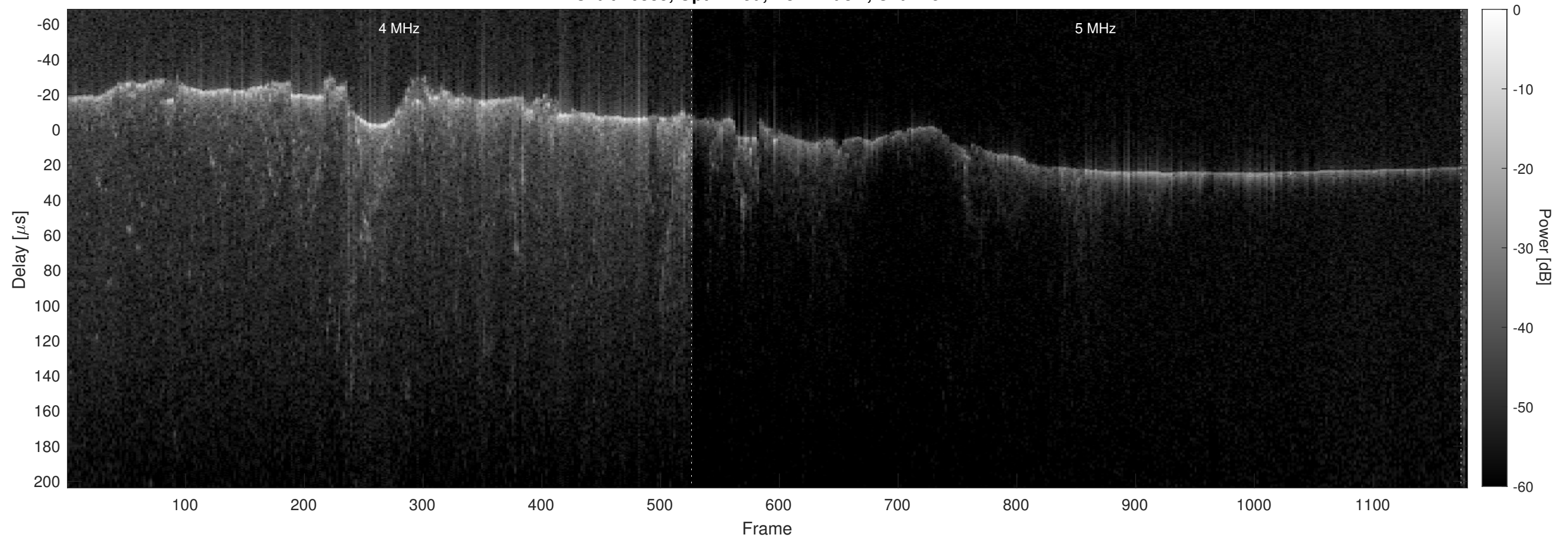
Orbit 10385, Optimized, No Window, Channel 2
