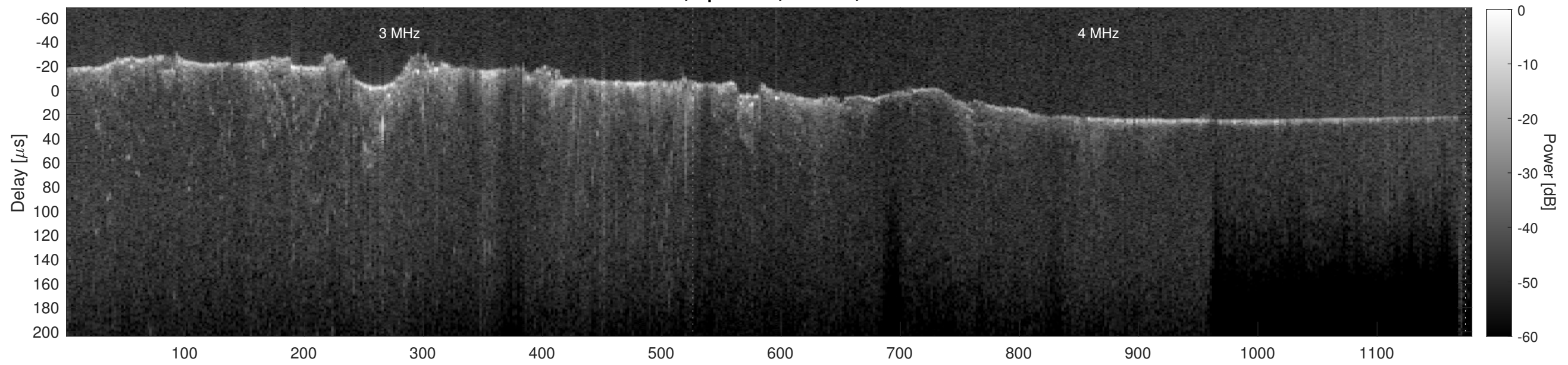
Orbit 10385, Cluttergram
