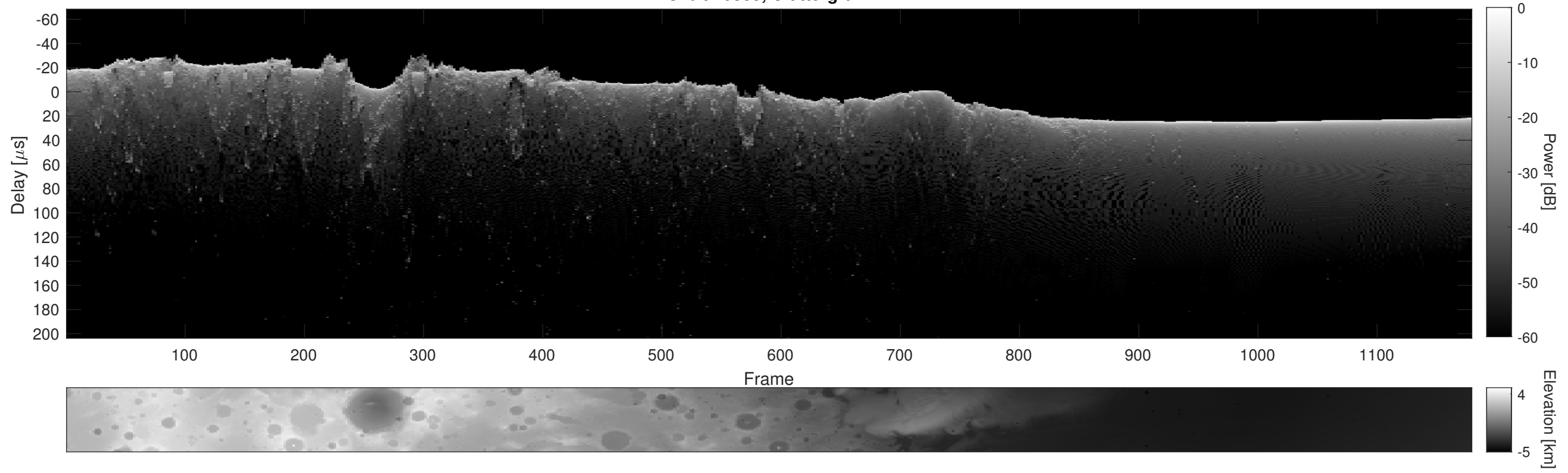
Orbit 10385, Cluttergram
