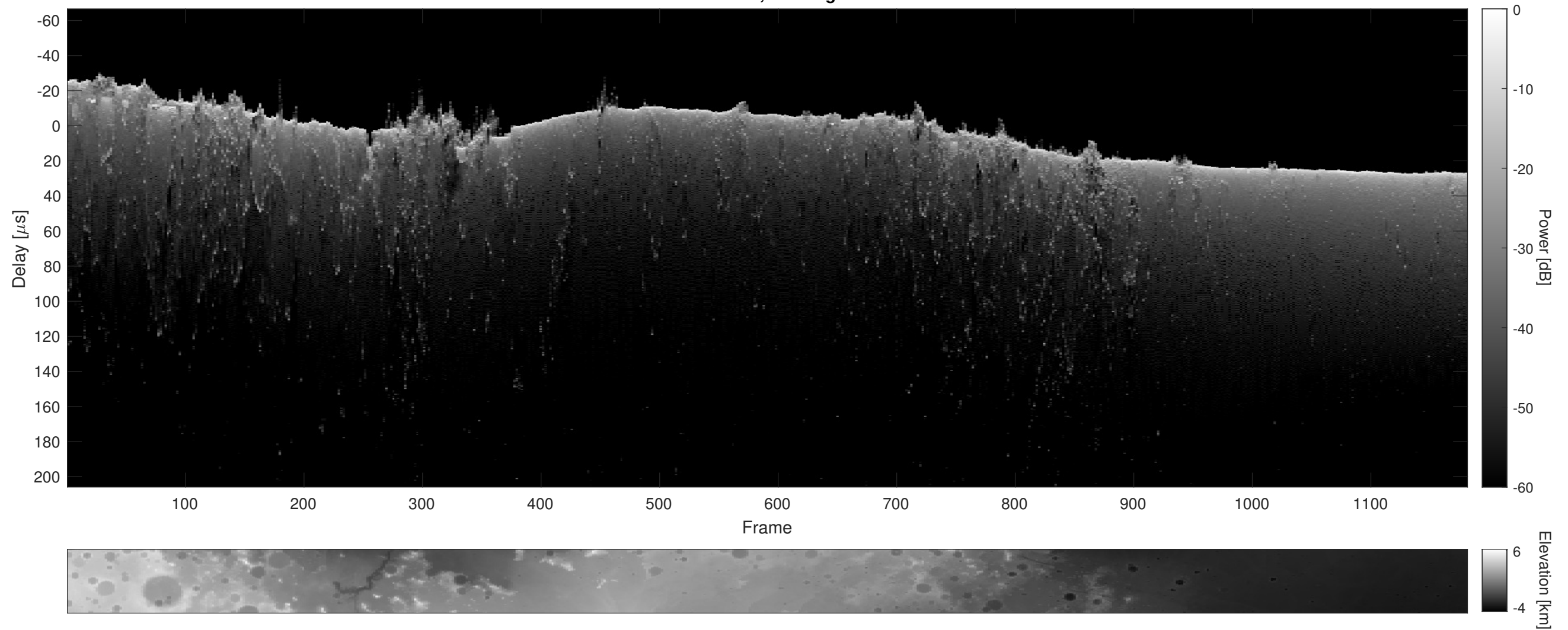
Orbit 10386, Cluttergram
