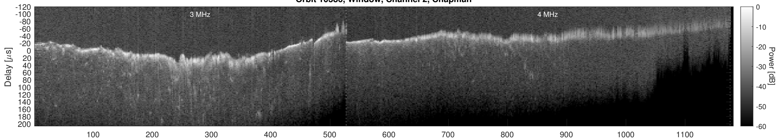
Orbit 10386, Window, Channel 2, Optimized
