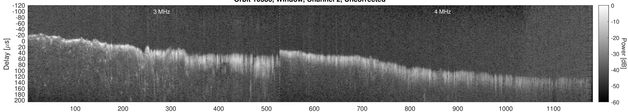
Orbit 10386, Window, Channel 2, Chapman
