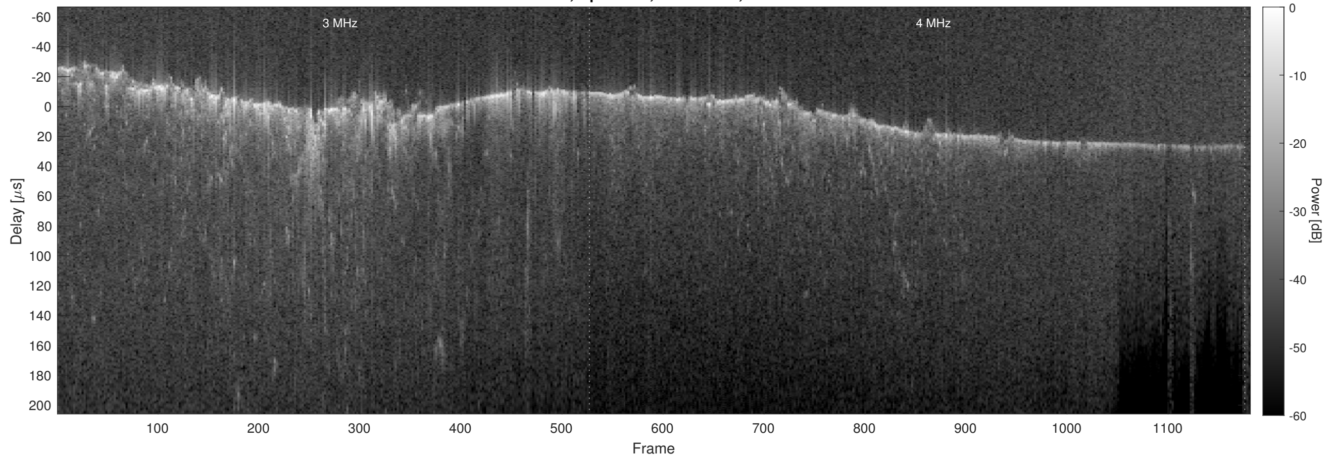
Orbit 10386, Optimized, No Window, Channel 2
