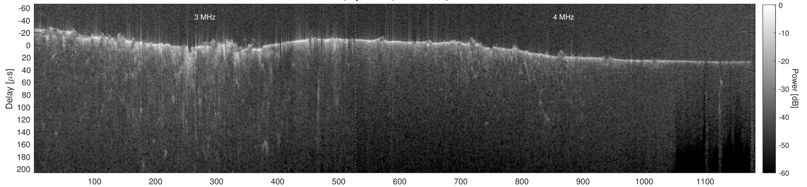
Orbit 10386, Cluttergram
