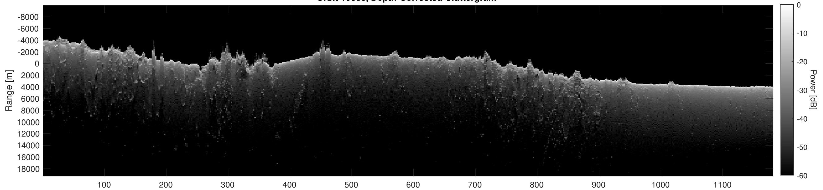
Orbit 10386, Depth-Corrected Cluttergram
