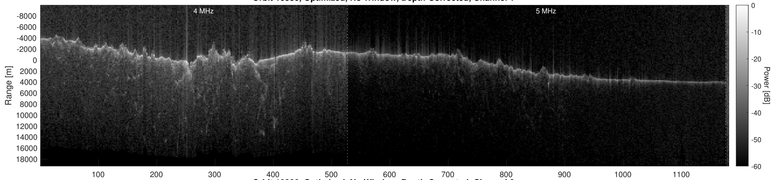
Orbit 10386, Optimized, No Window, Depth-Corrected, Channel 2
