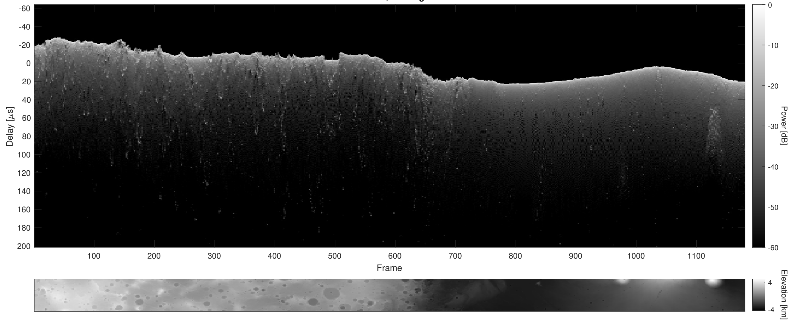
Orbit 10389, Cluttergram
