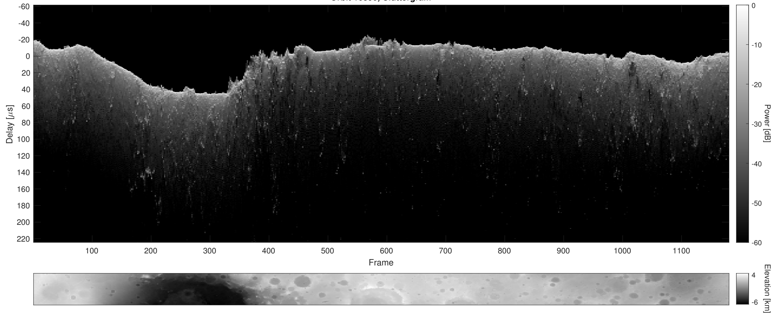
Orbit 10390, Cluttergram
