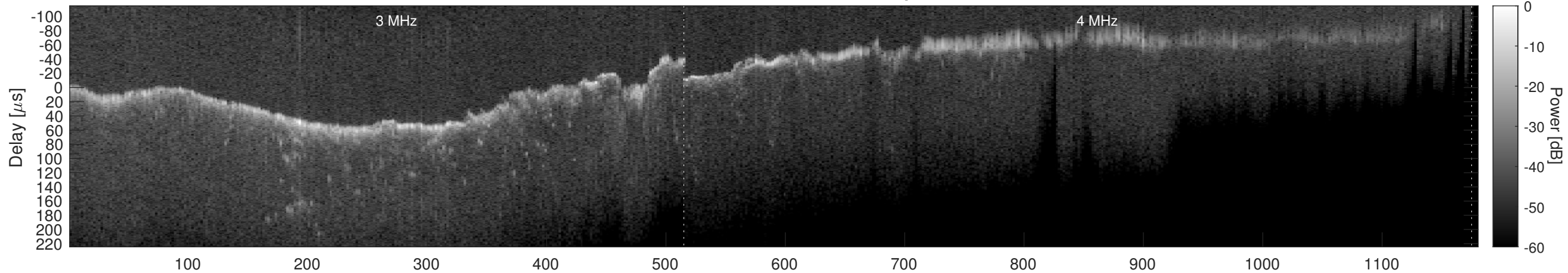
Orbit 10390, Window, Channel 2, Optimized
