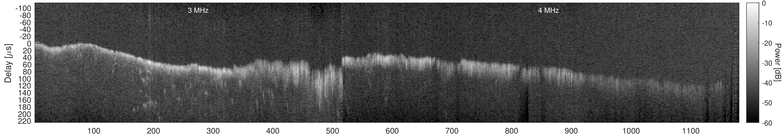
Orbit 10390, Window, Channel 2, Chapman
