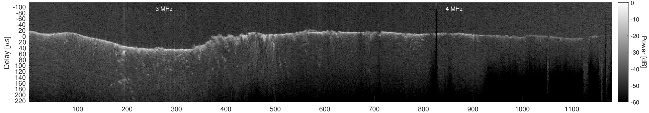
Orbit 10390, Cluttergram
