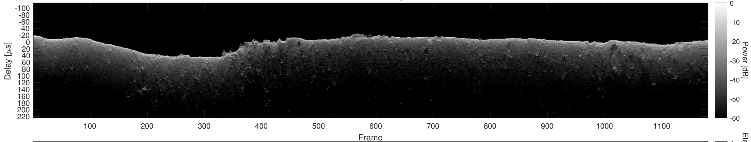
Orbit 10390, Cluttergram
