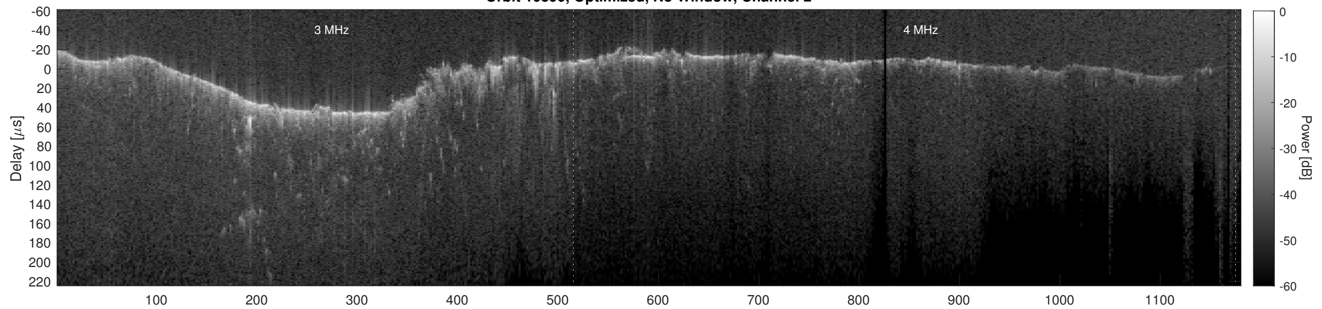
Orbit 10390, Cluttergram
