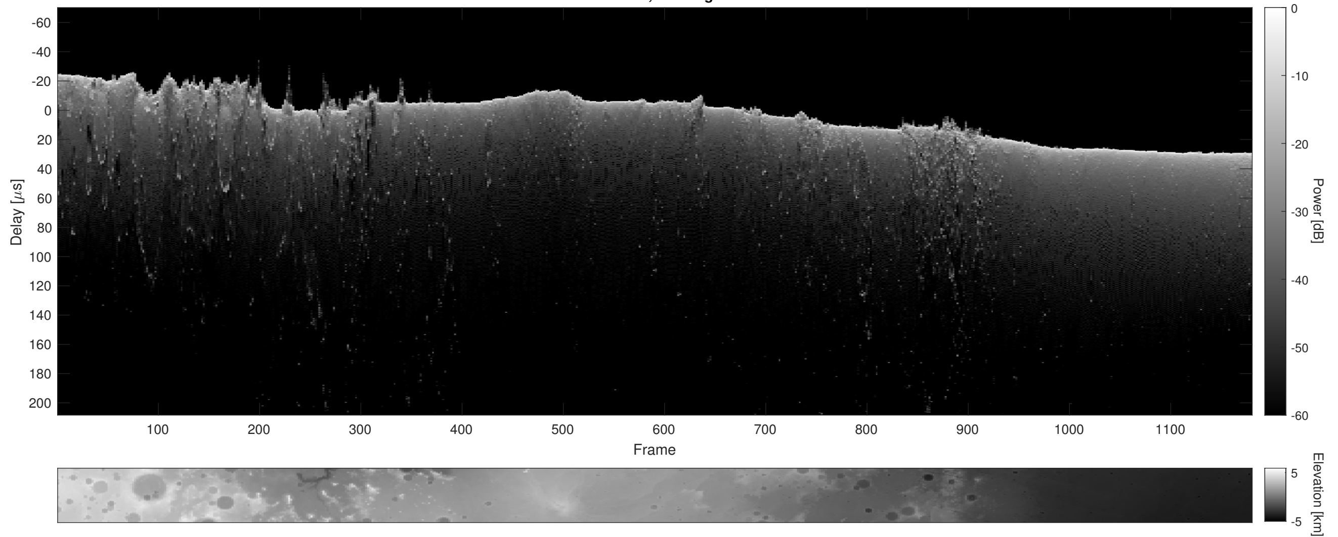
Orbit 10393, Cluttergram
