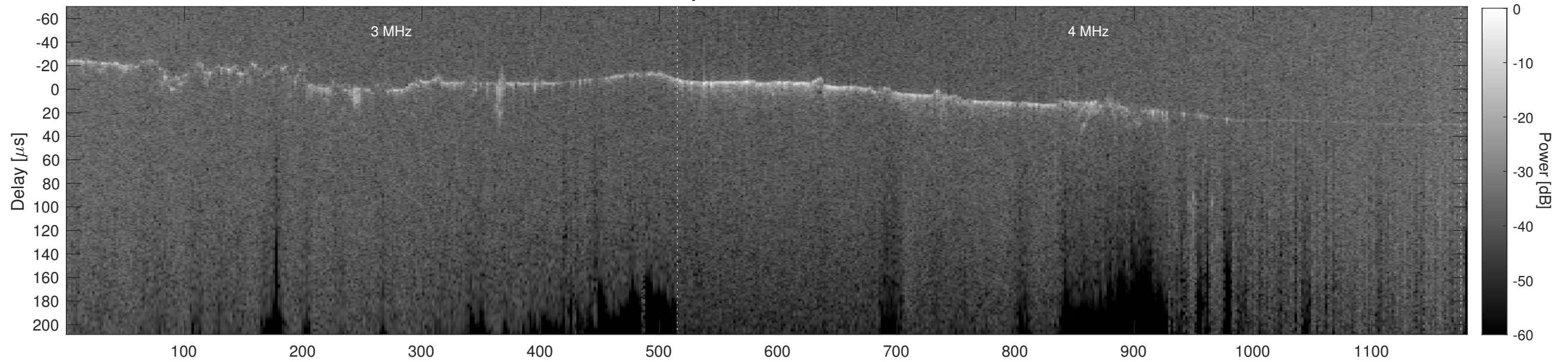
Orbit 10393, Cluttergram
