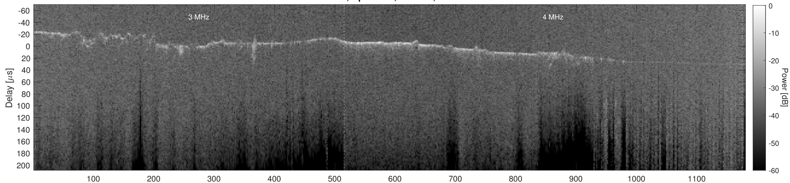
Orbit 10393, Cluttergram
