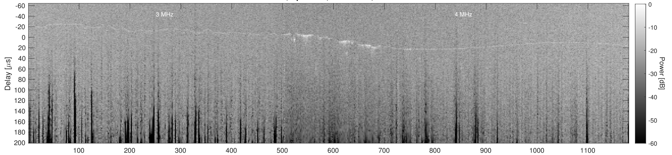
Orbit 10396, Cluttergram
