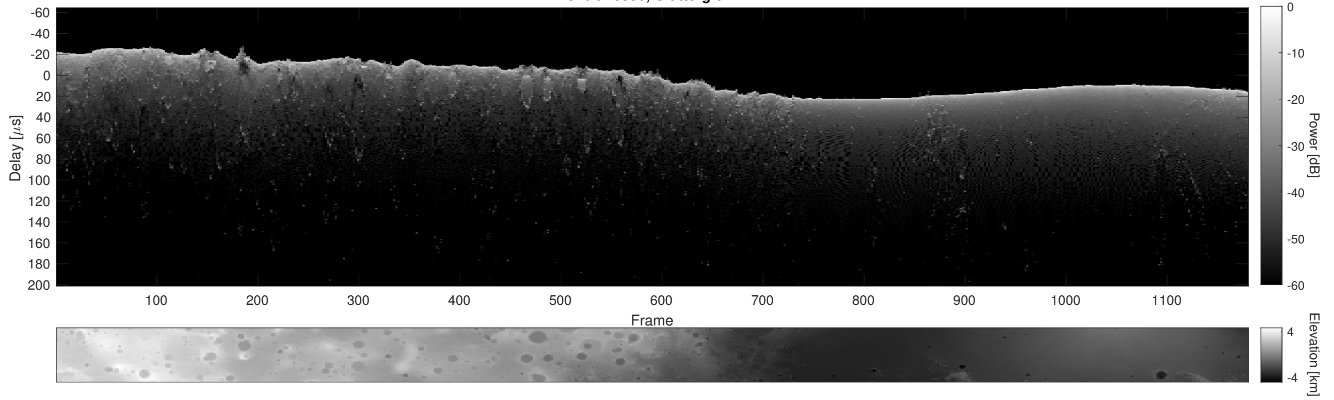
Orbit 10396, Cluttergram
