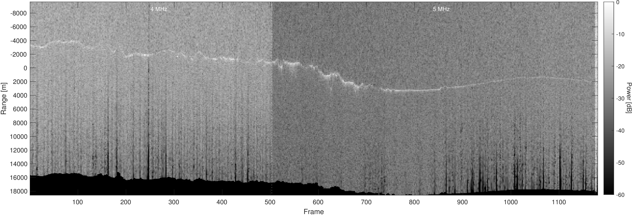
Orbit 10396, Optimized, No Window, Depth-Corrected, Channel 2
