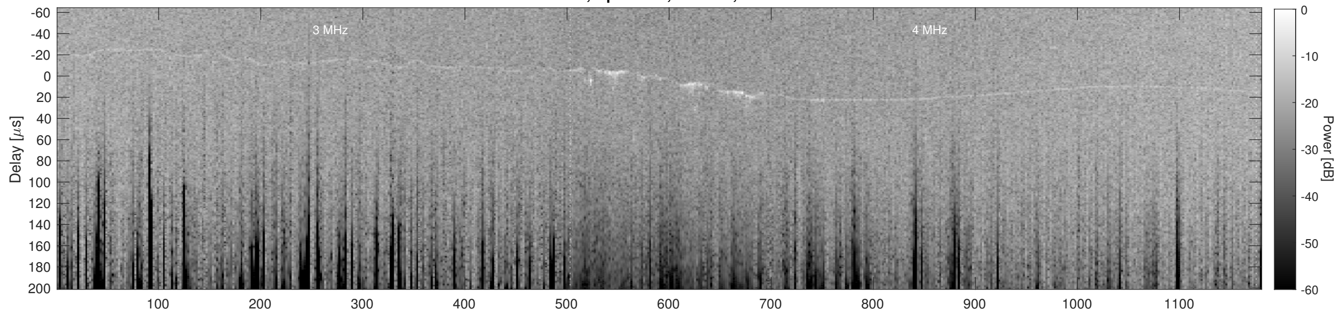
Orbit 10396, Cluttergram
