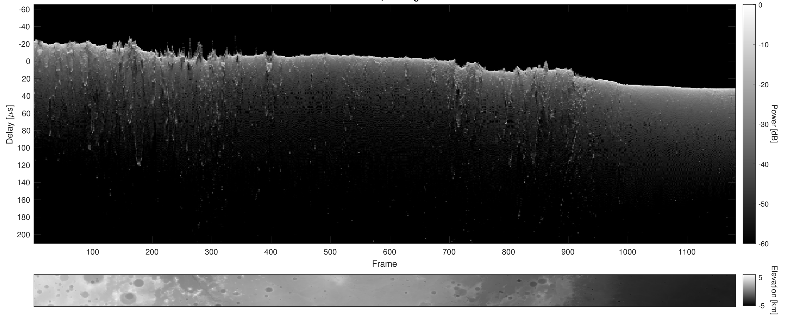
Orbit 10400, Cluttergram
