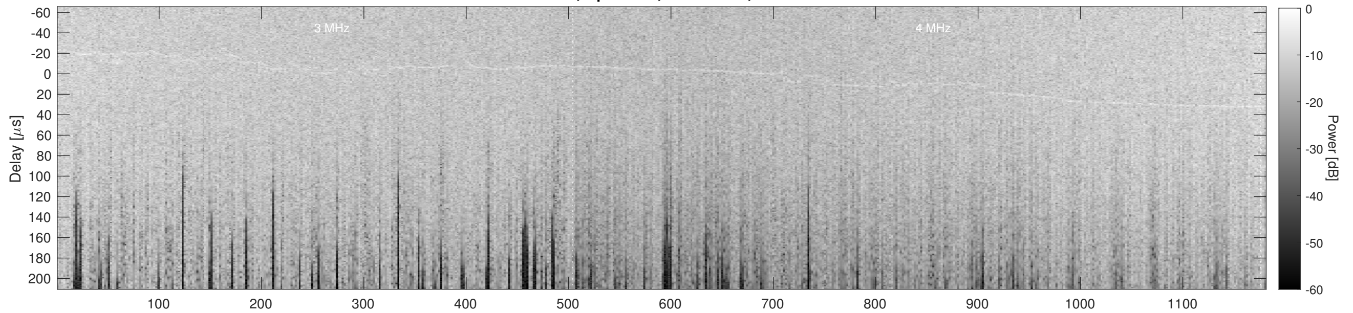
Orbit 10400, Cluttergram
