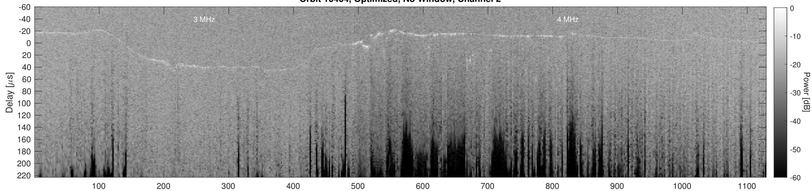
Orbit 10404, Cluttergram
