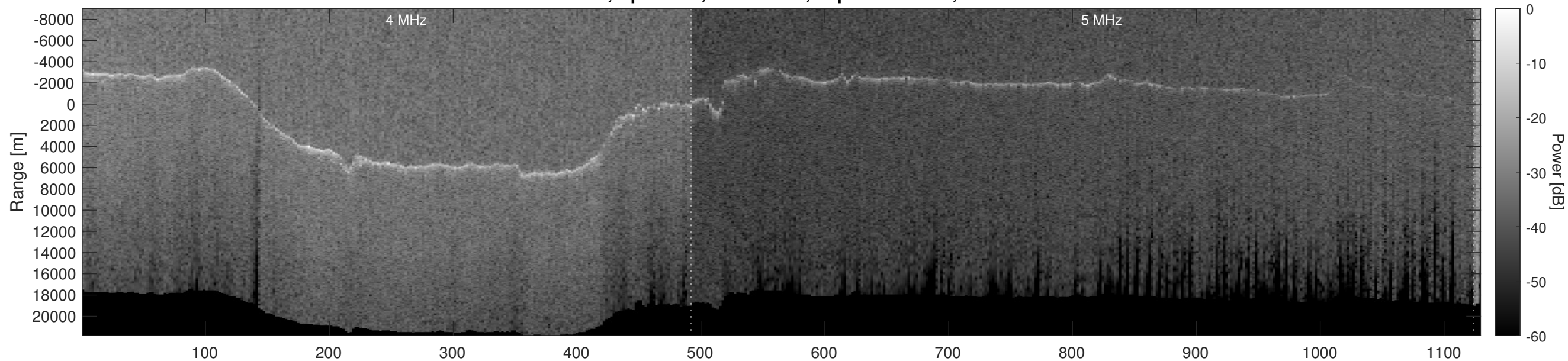
Orbit 10404, Optimized, No Window, Depth-Corrected, Channel 2
