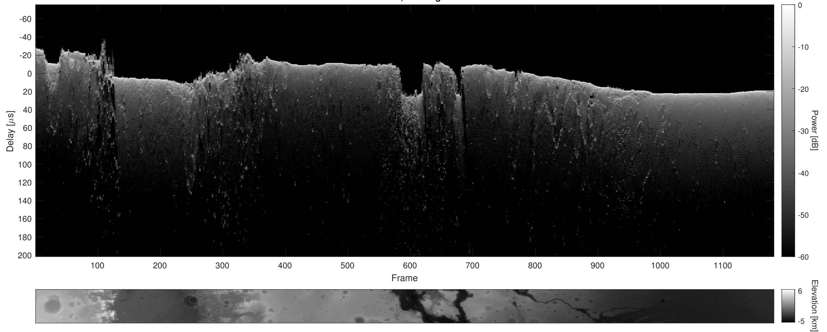
Orbit 10405, Cluttergram
