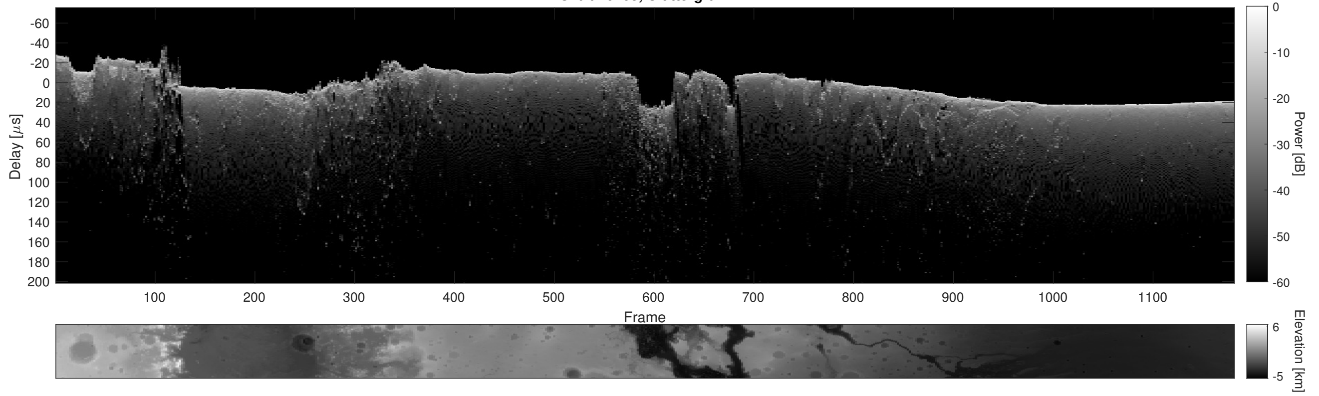
Orbit 10405, Cluttergram
