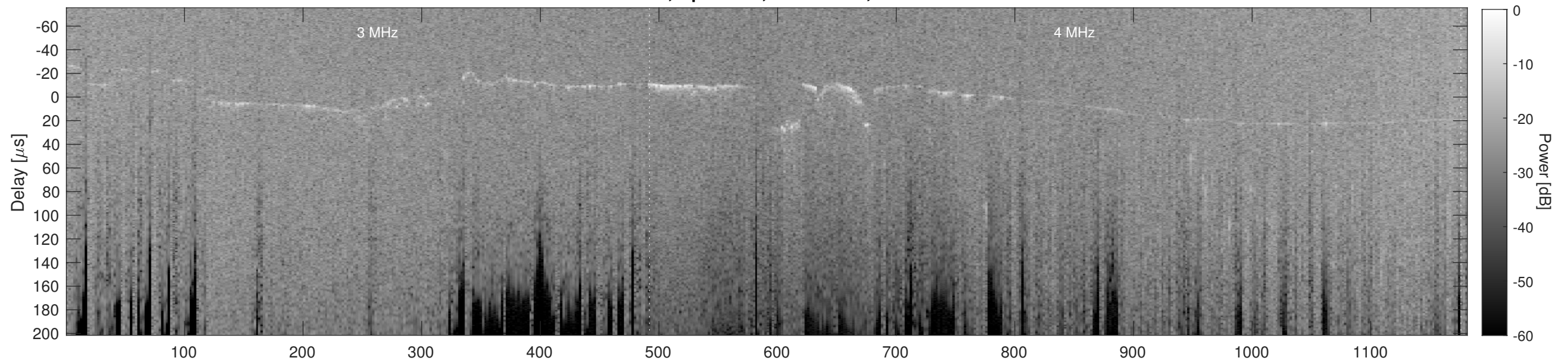
Orbit 10405, Cluttergram
