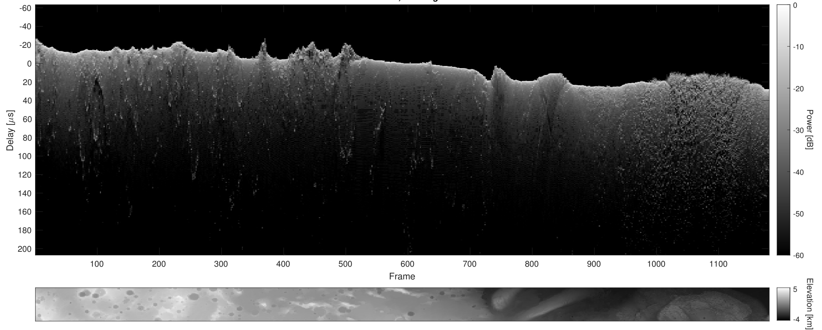
Orbit 10406, Cluttergram
