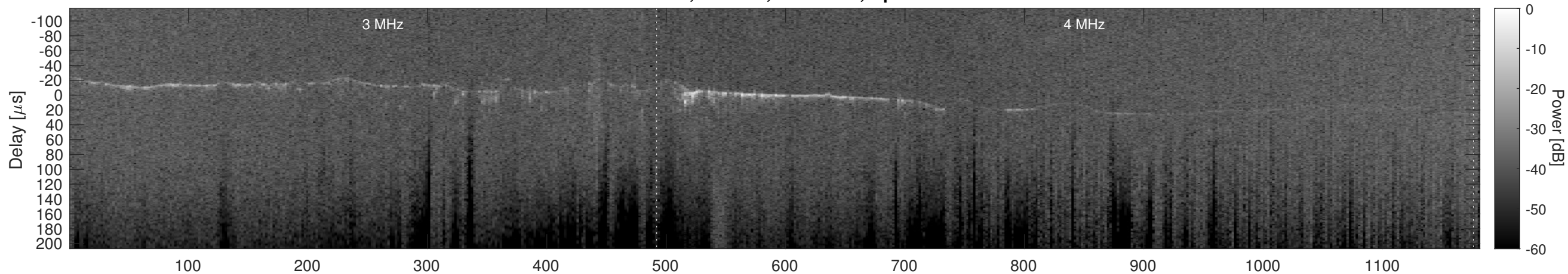
Orbit 10406, Cluttergram
