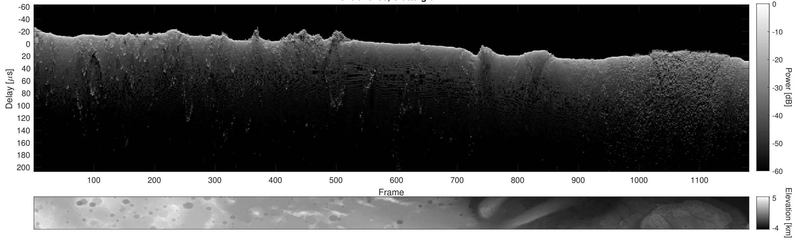
Orbit 10406, Cluttergram
