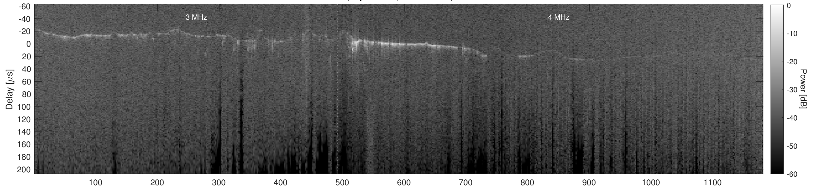
Orbit 10406, Cluttergram
