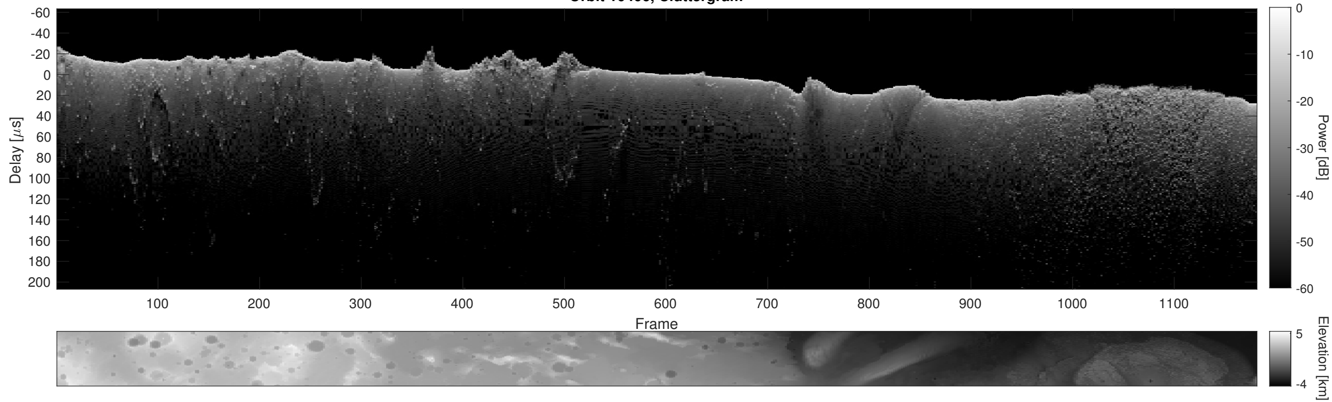
Orbit 10406, Cluttergram
