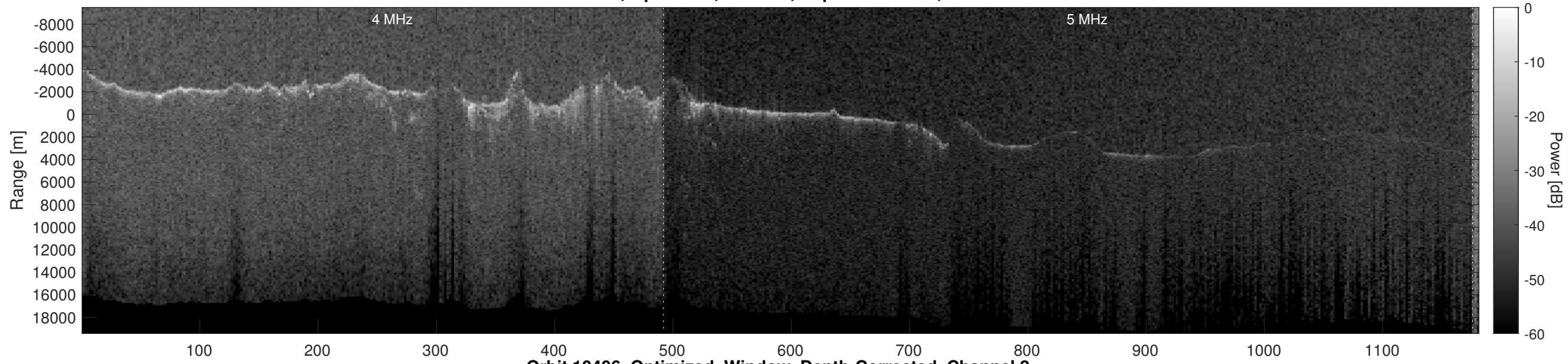
Orbit 10406, Optimized, Window, Depth-Corrected, Channel 2
