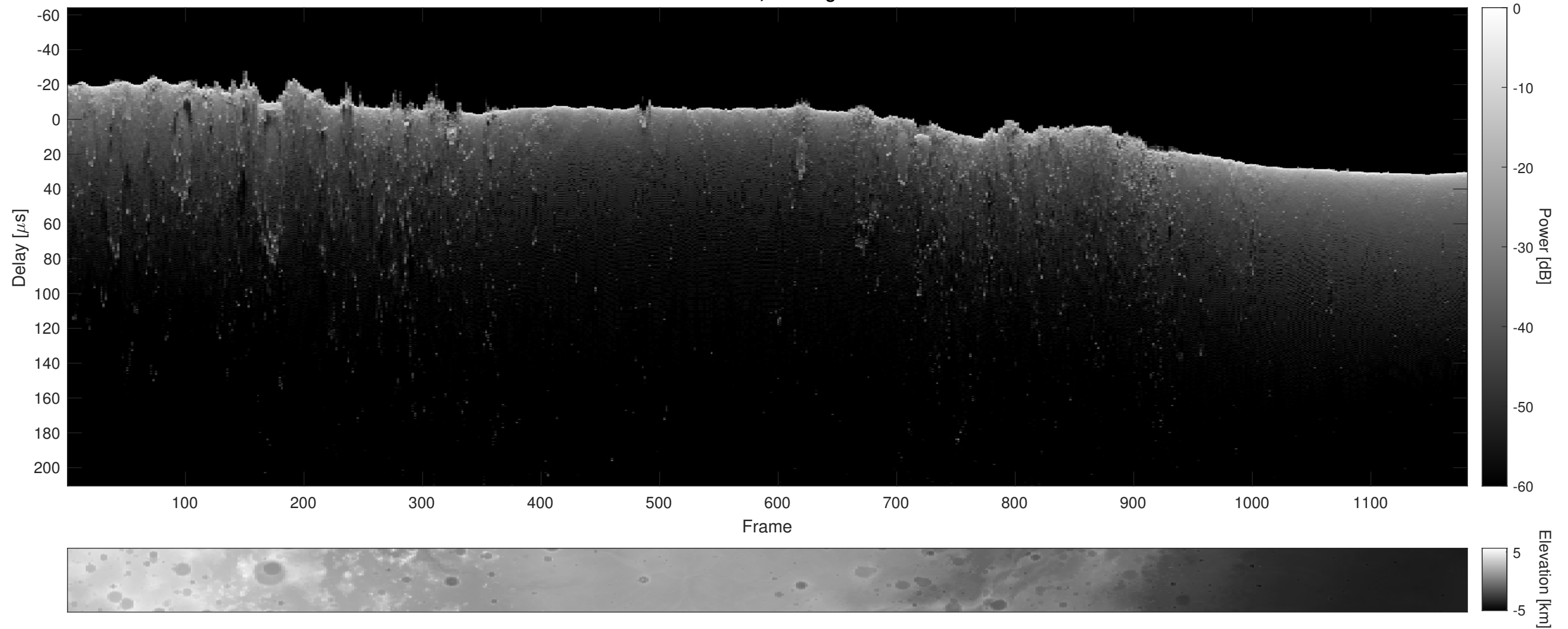
Orbit 10407, Cluttergram
