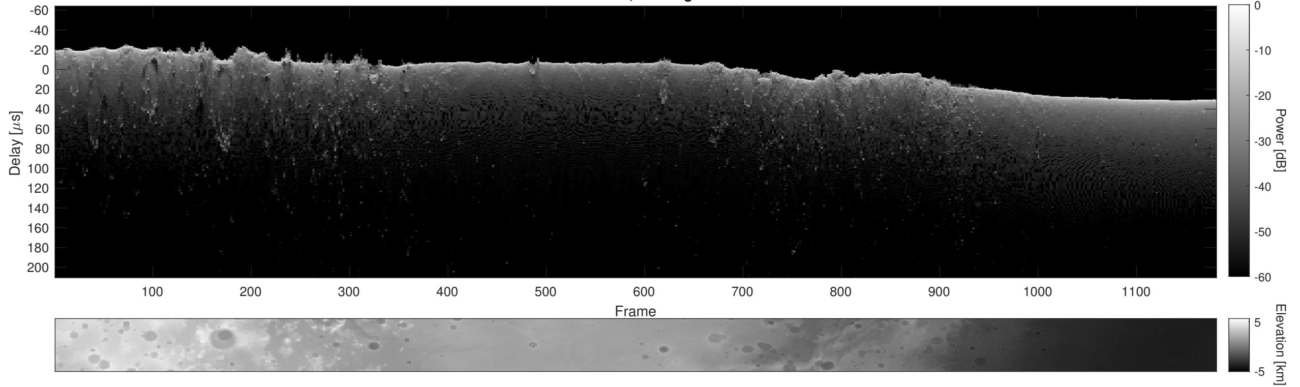
Orbit 10407, Cluttergram
