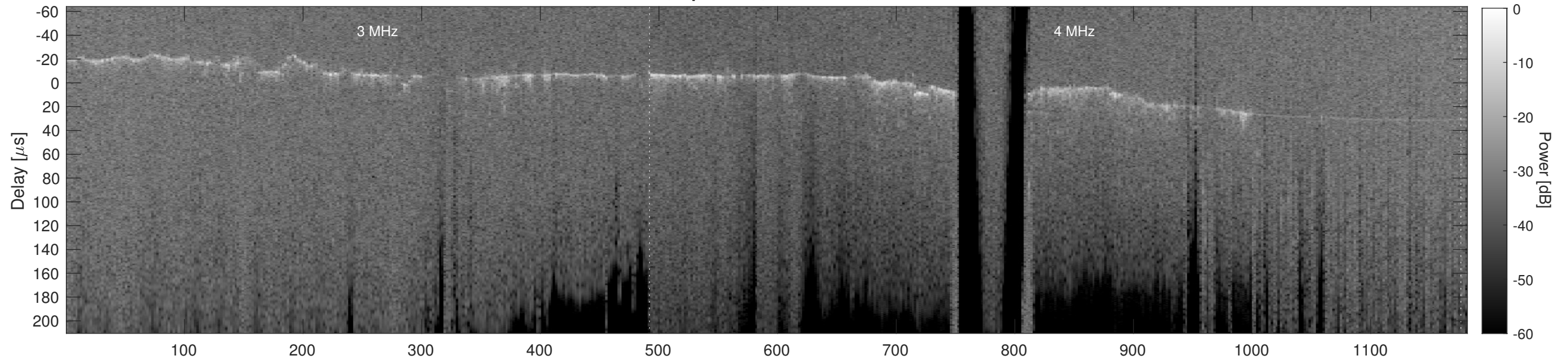
Orbit 10407, Cluttergram
