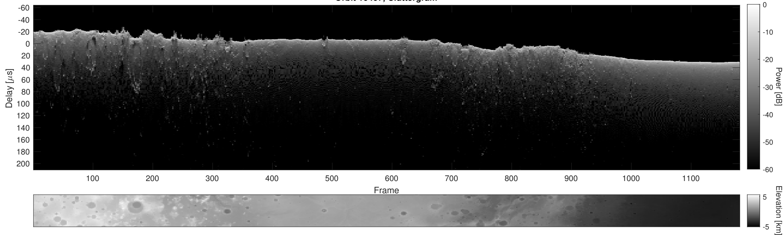
Orbit 10407, Cluttergram
