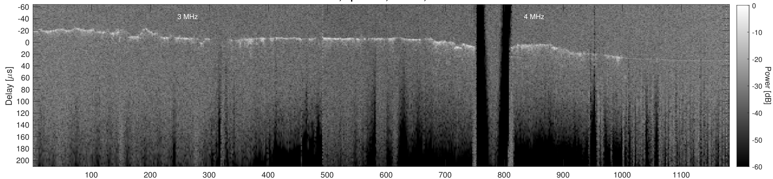
Orbit 10407, Cluttergram
