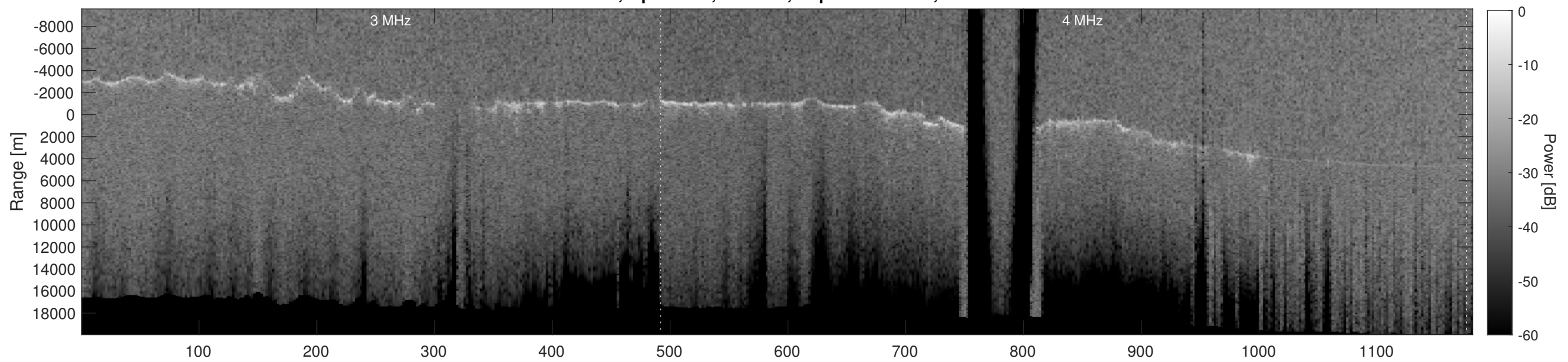
Orbit 10407, Depth-Corrected Cluttergram
