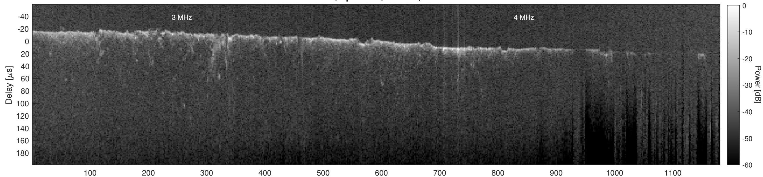
Orbit 10408, Cluttergram
