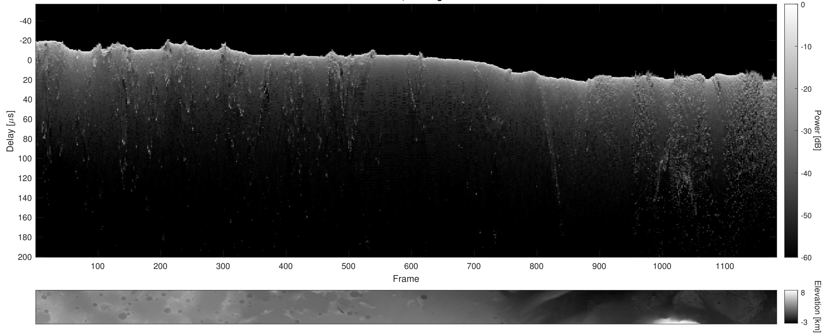
Orbit 10413, Cluttergram
