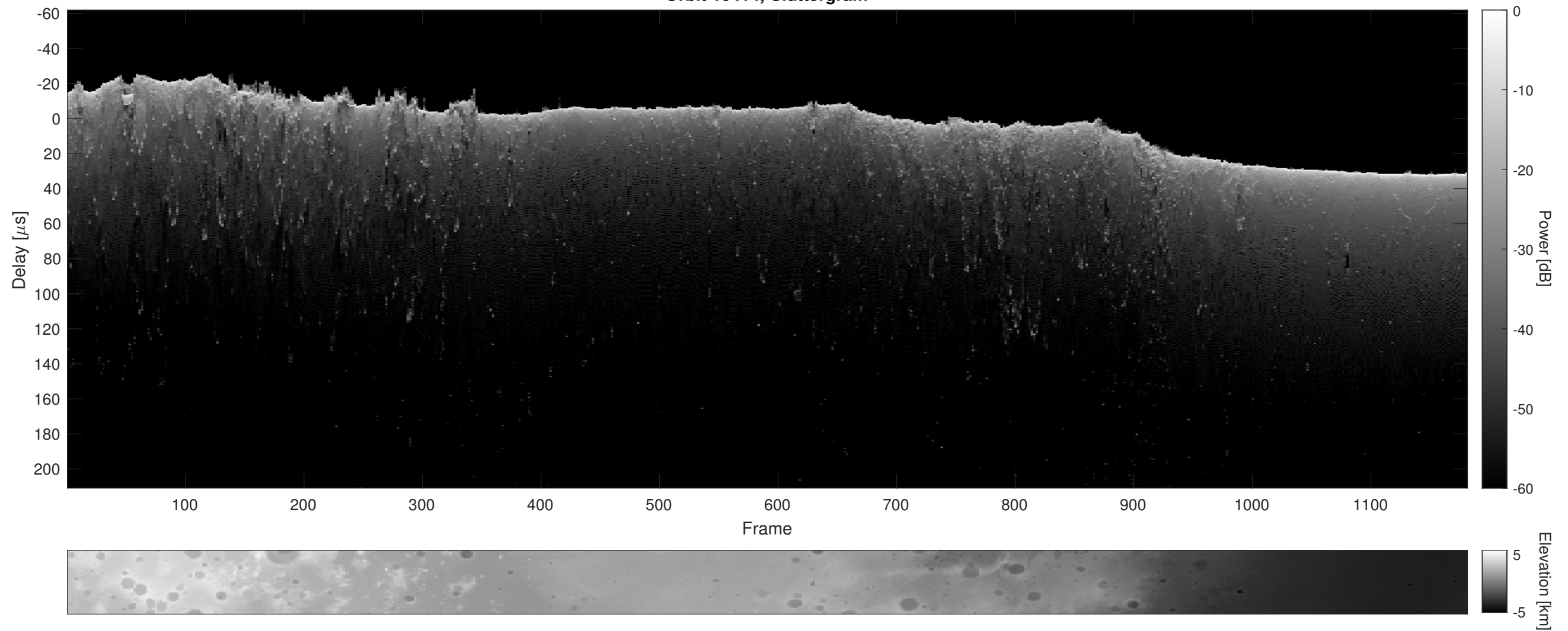
Orbit 10414, Cluttergram
