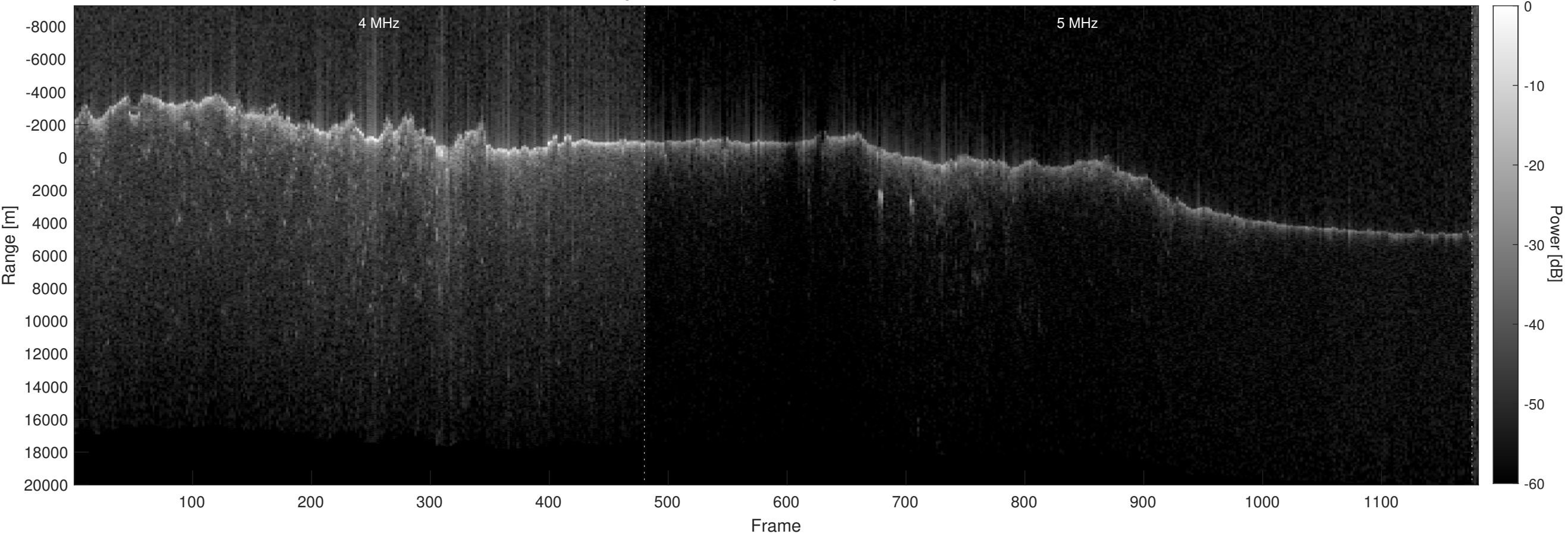
Orbit 10414, Optimized, No Window, Depth-Corrected, Channel 2
