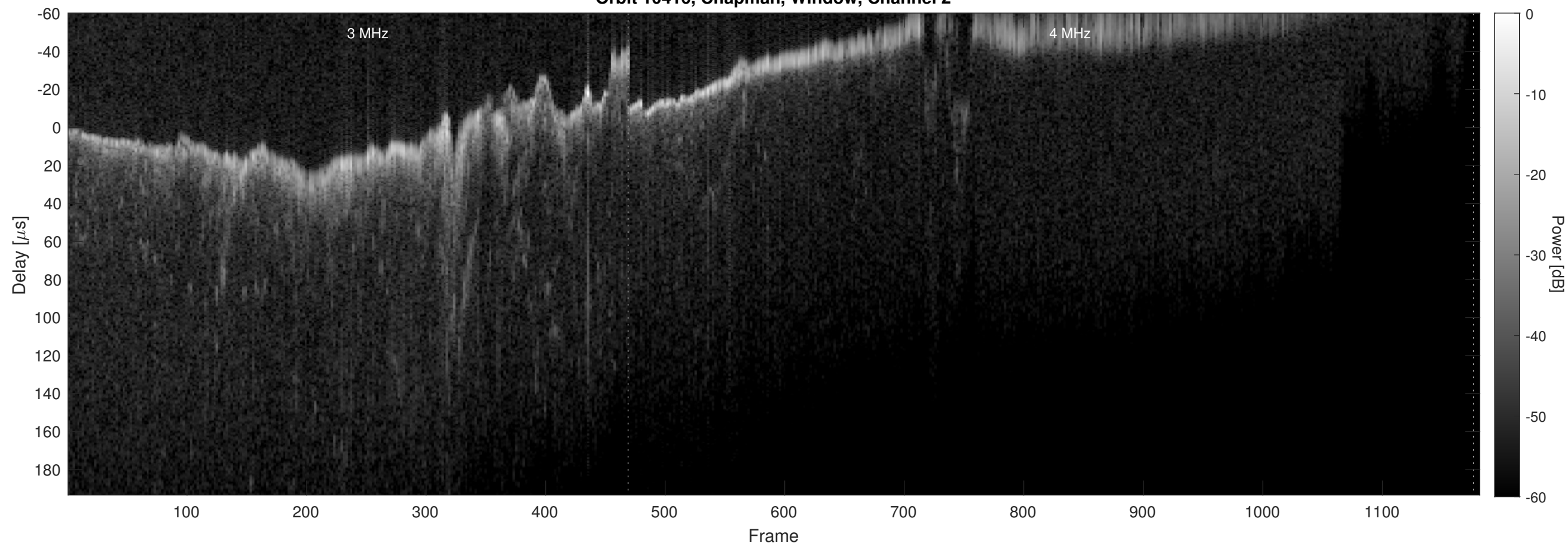
Orbit 10416, Chapman, Window, Channel 2
