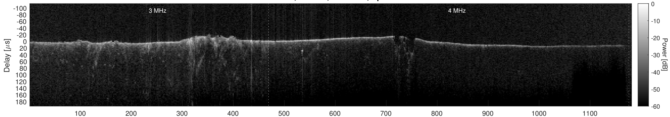
Orbit 10416, Cluttergram
