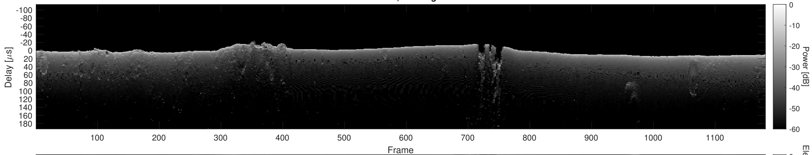
Orbit 10416, Cluttergram
