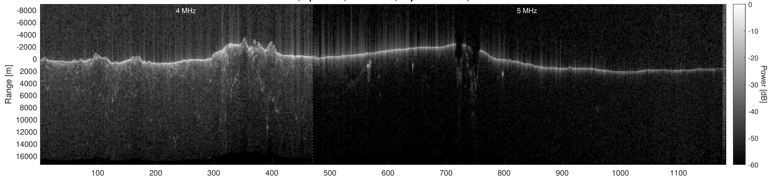
Orbit 10416, Optimized, No Window, Depth-Corrected, Channel 2
