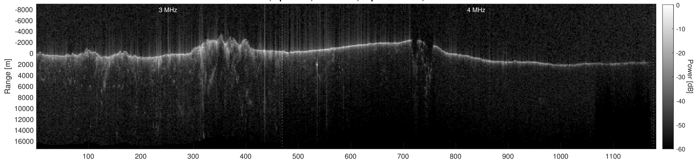
Orbit 10416, Depth-Corrected Cluttergram
