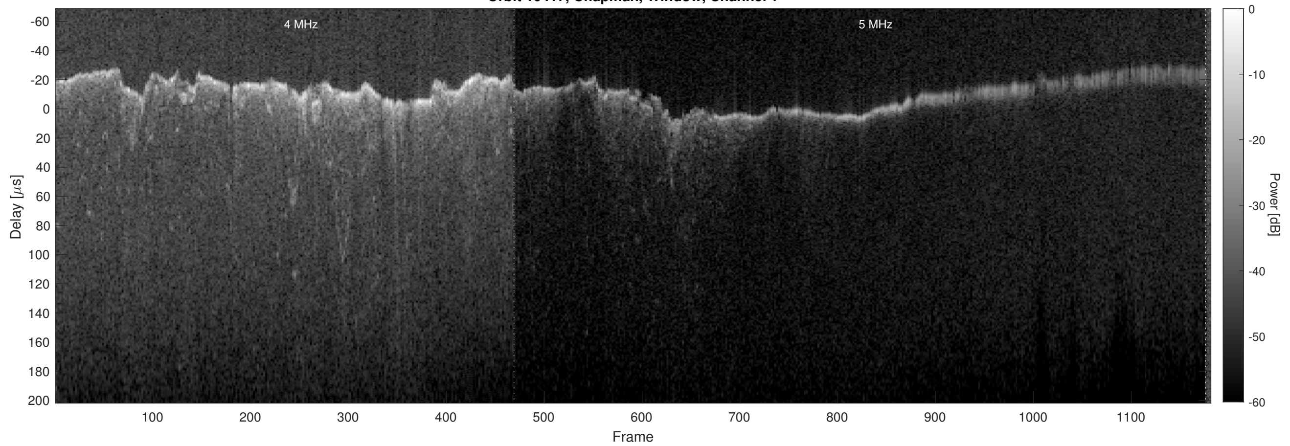
Orbit 10417, Chapman, Window, Channel 2
