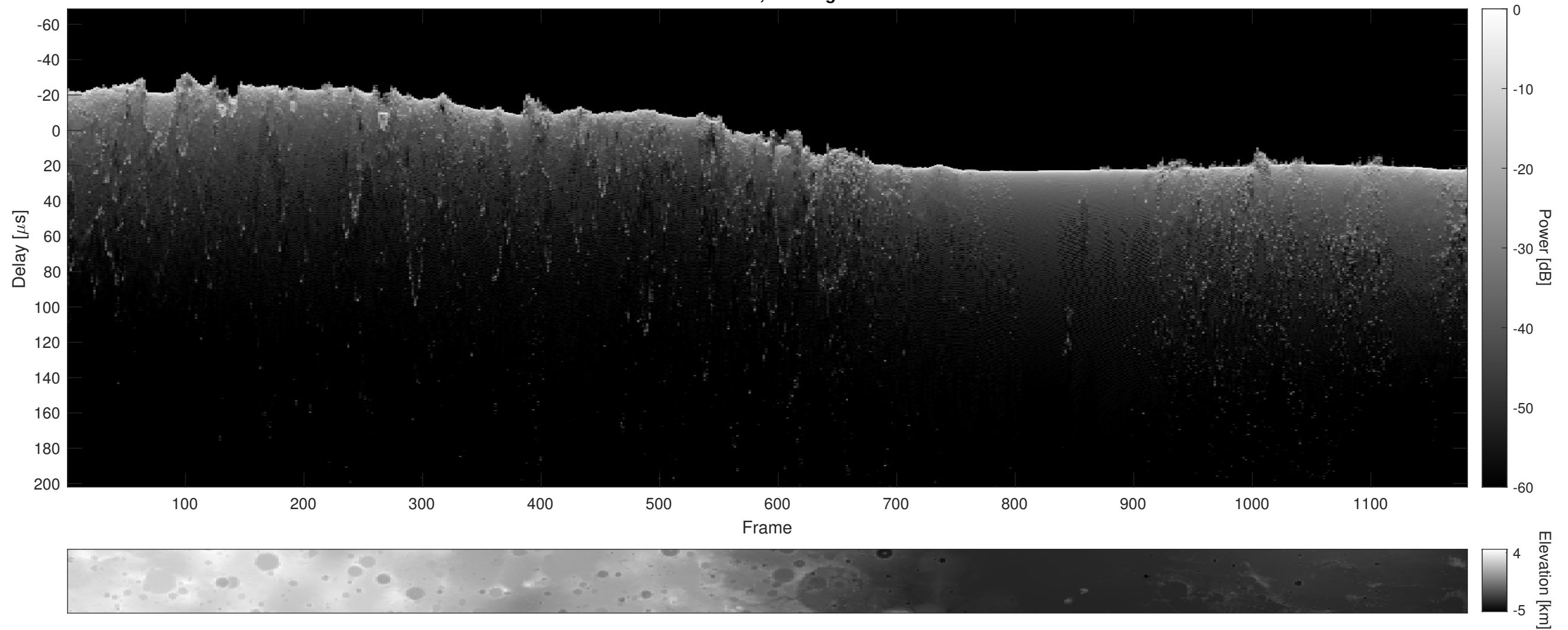
Orbit 10417, Cluttergram
