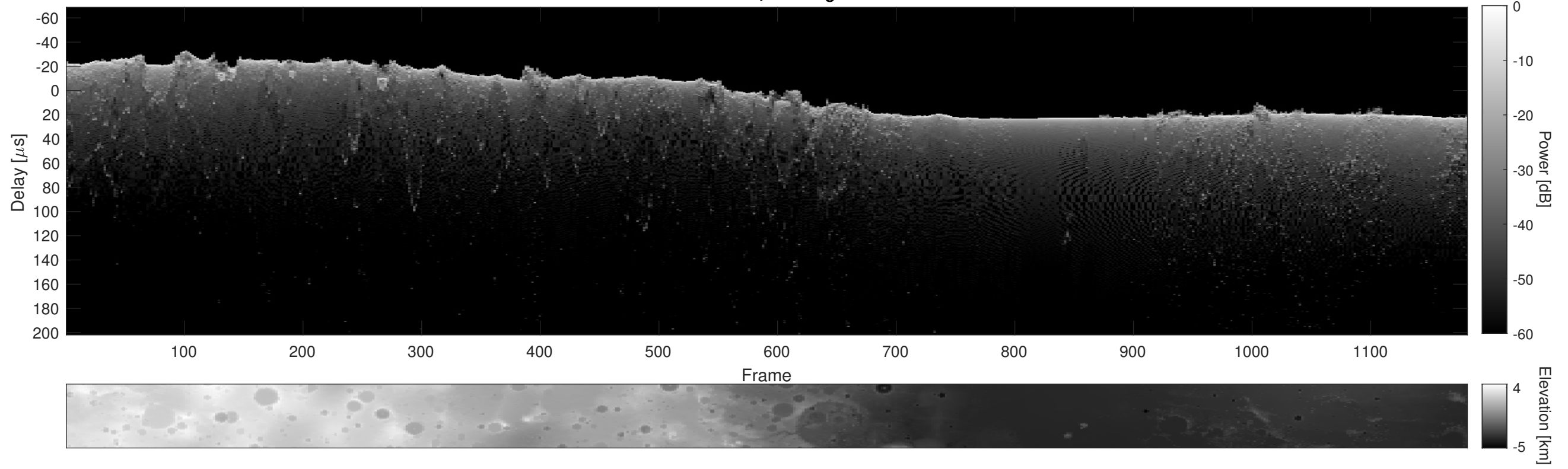
Orbit 10417, Cluttergram
