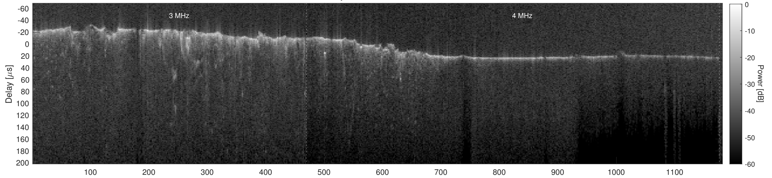
Orbit 10417, Cluttergram
