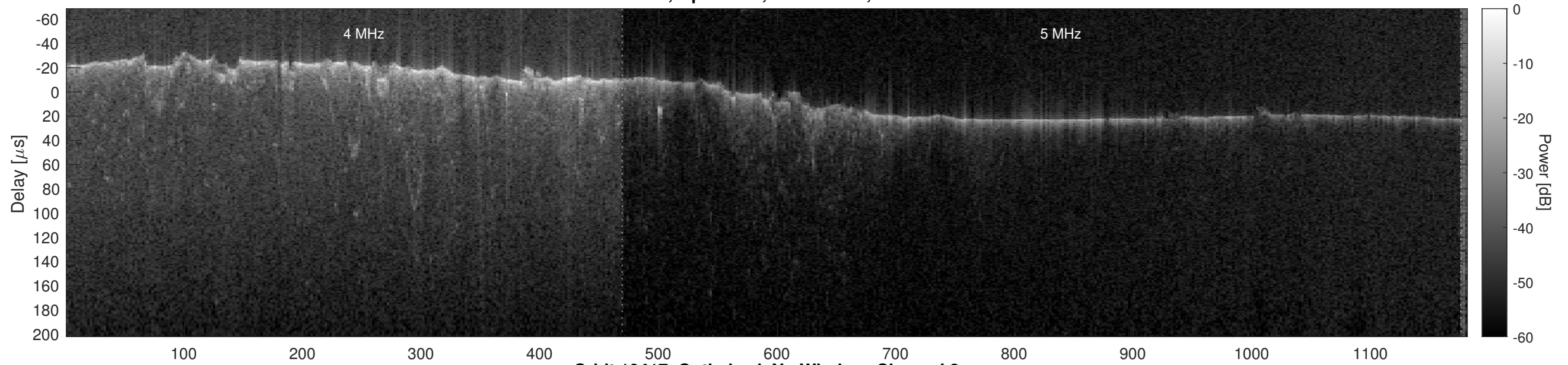
Orbit 10417, Optimized, No Window, Channel 2
