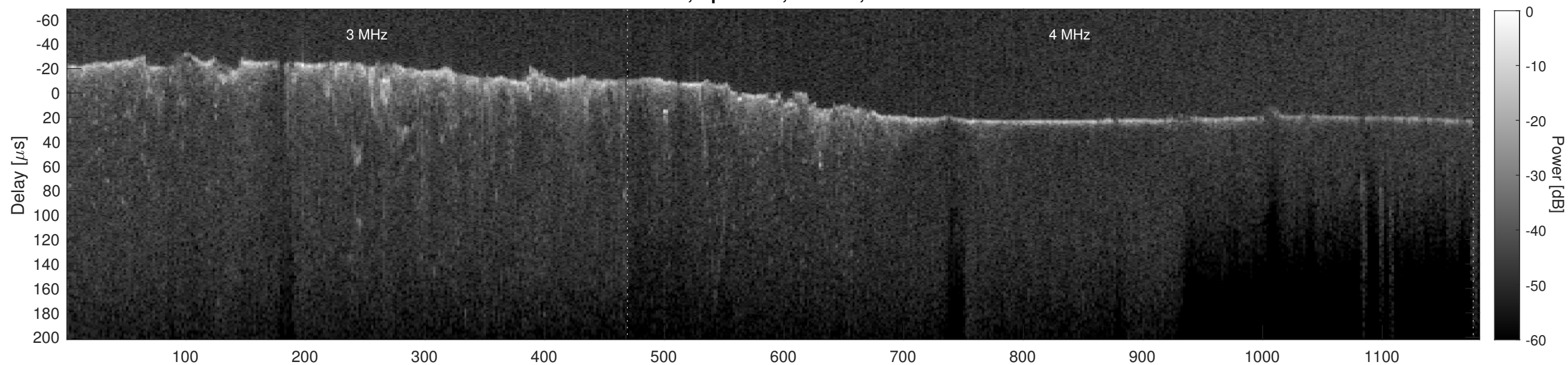
Orbit 10417, Cluttergram
