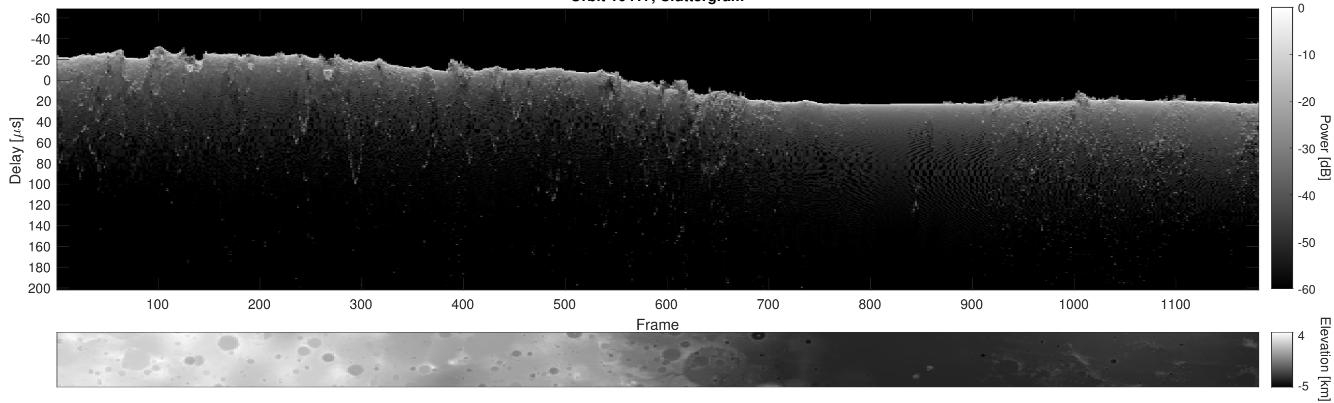
Orbit 10417, Cluttergram
