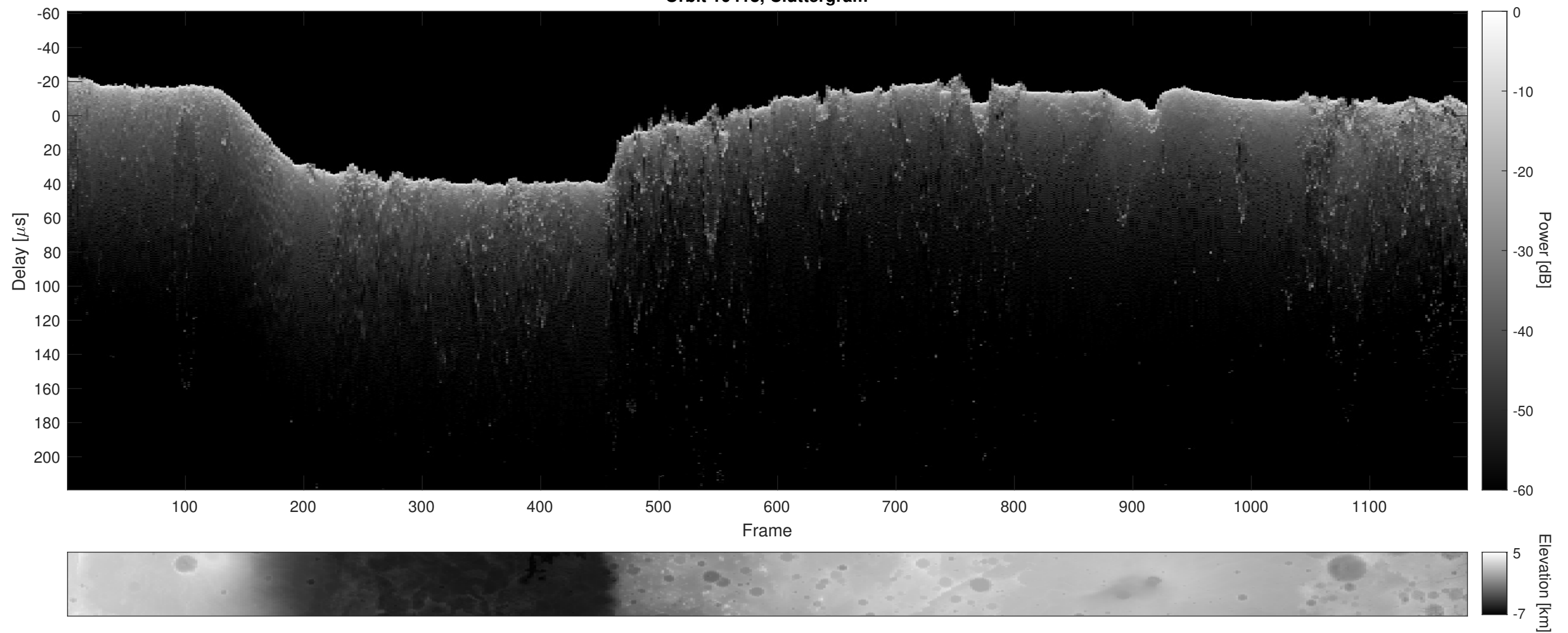
Orbit 10418, Cluttergram
