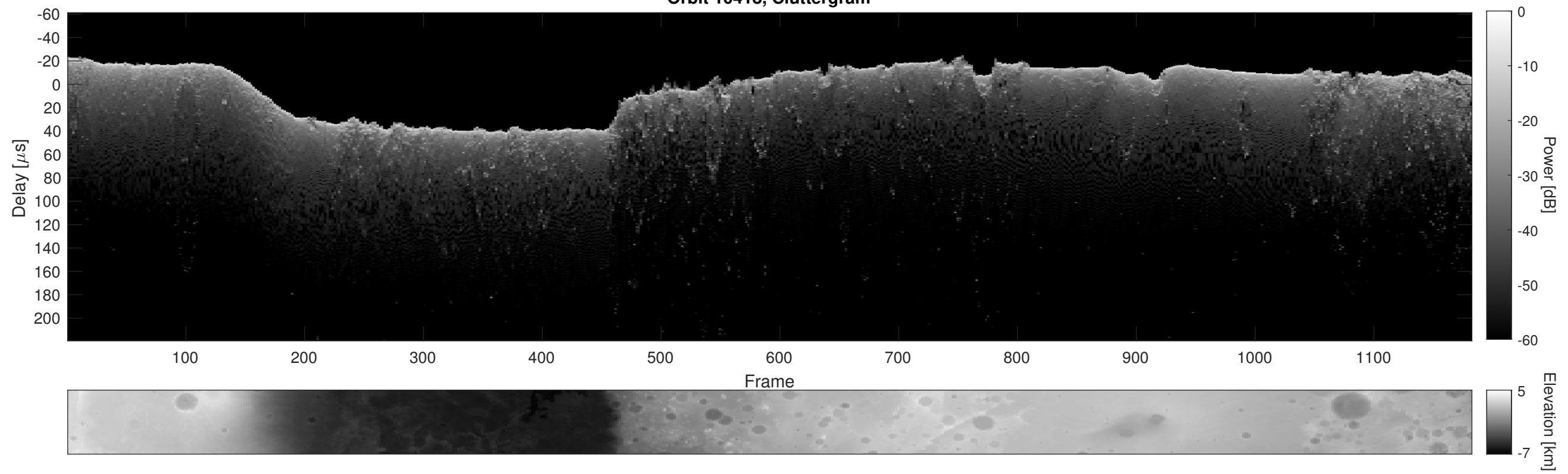
Orbit 10418, Cluttergram
